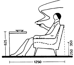
16 Dimensions: armchair
